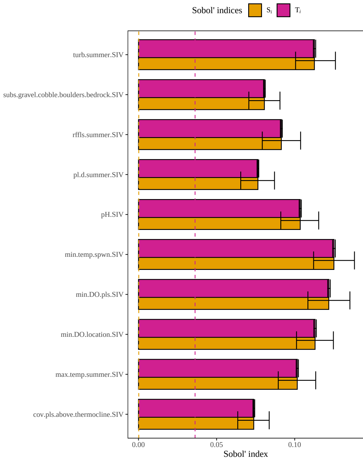
Figure 4. Results of a sensitivity analysis for the spottedbassRiv model based on an arithmetic mean structure. Dashed lines represent baseline numerical approximation error for S_i and T_i ( i.e. , dummy variables).
