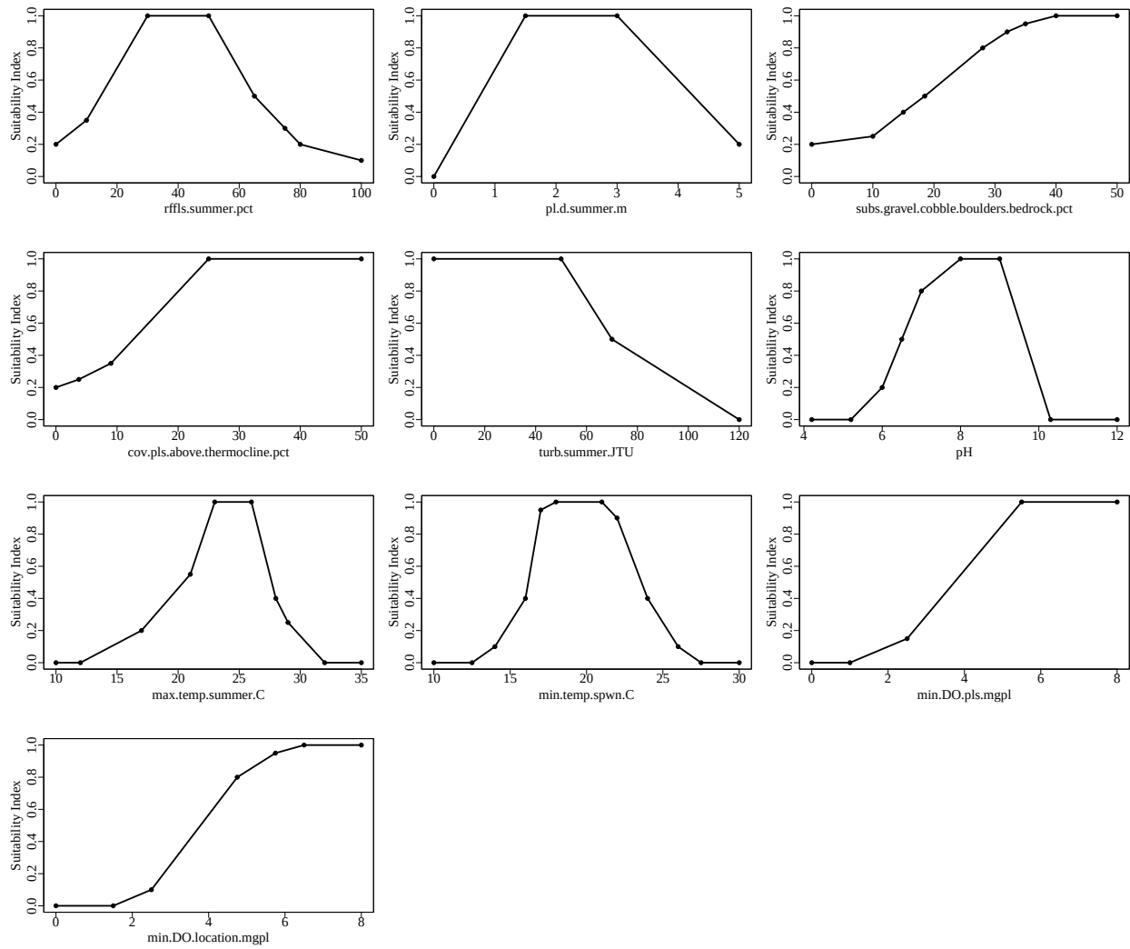
Figure 1. Suitability index graphs for variables included in the spottedbassRiv model in ecorest.
